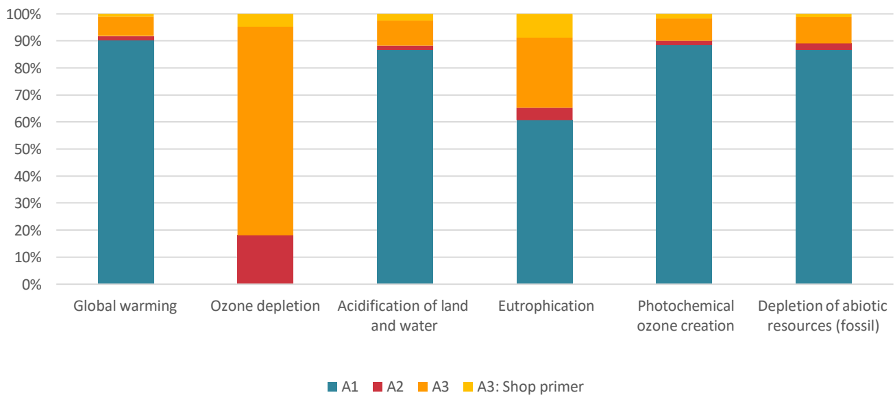
Figure 2: Relative contributions of the life cycle stages of the painted fabricated structural steel plates
